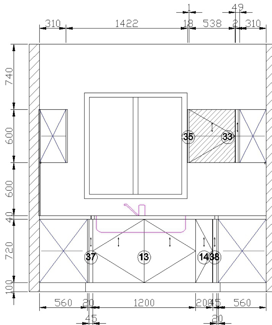
C View elevation drawing
