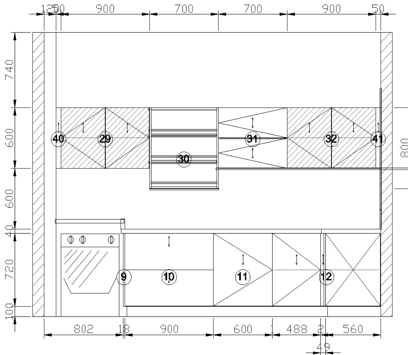
B View elevation drawing
