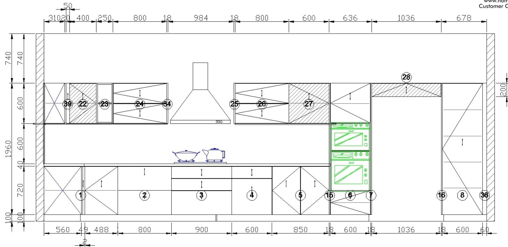
A View elevation drawing
