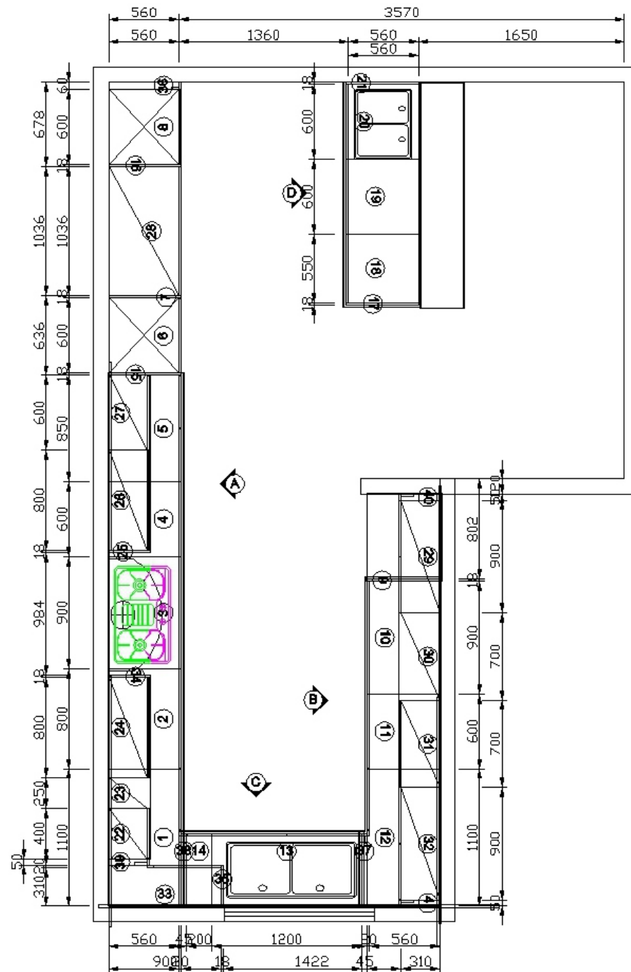
Plan drawing
